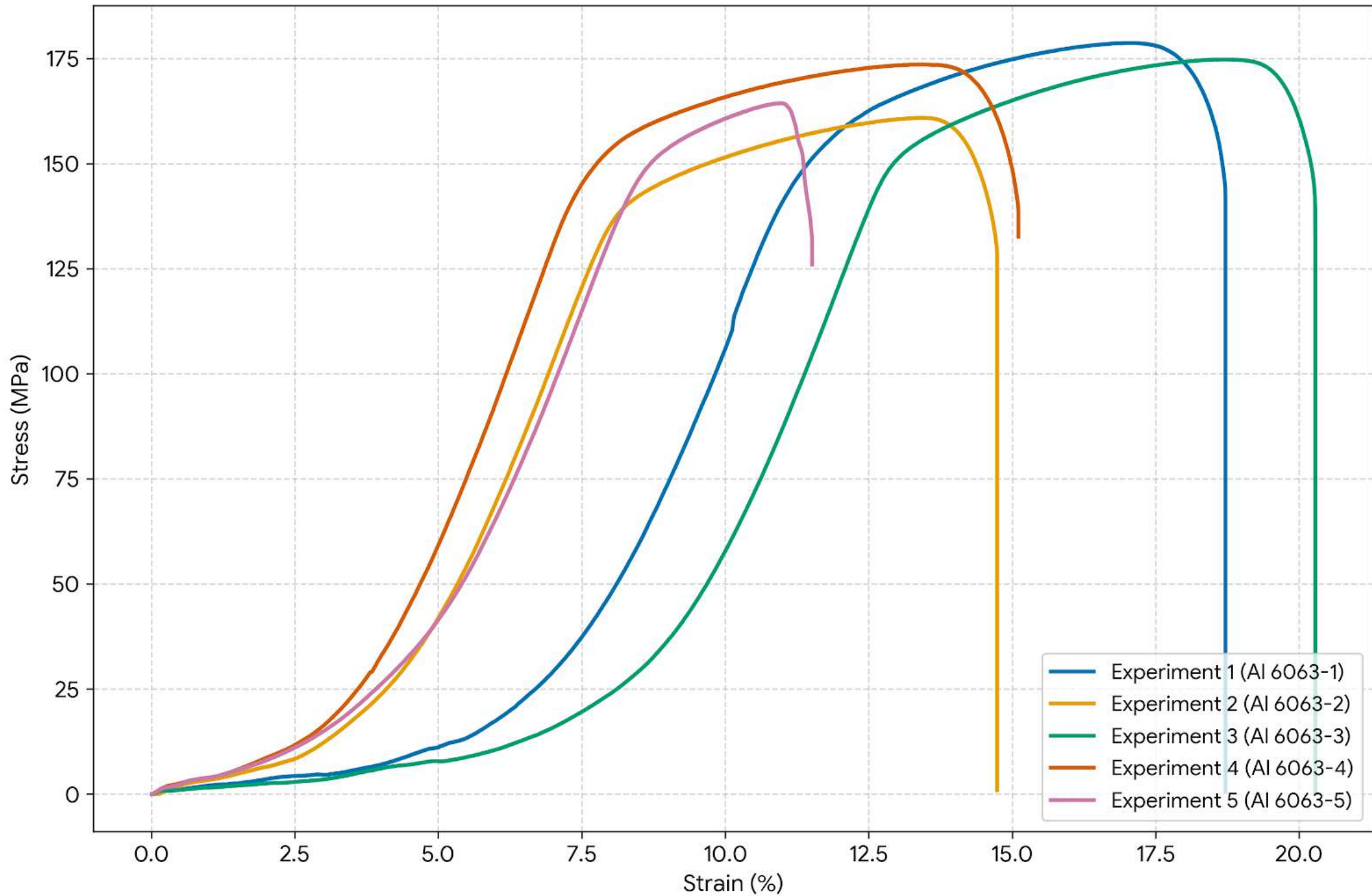
Stress-Strain Curves for Al 6063 (5 Experiments)
